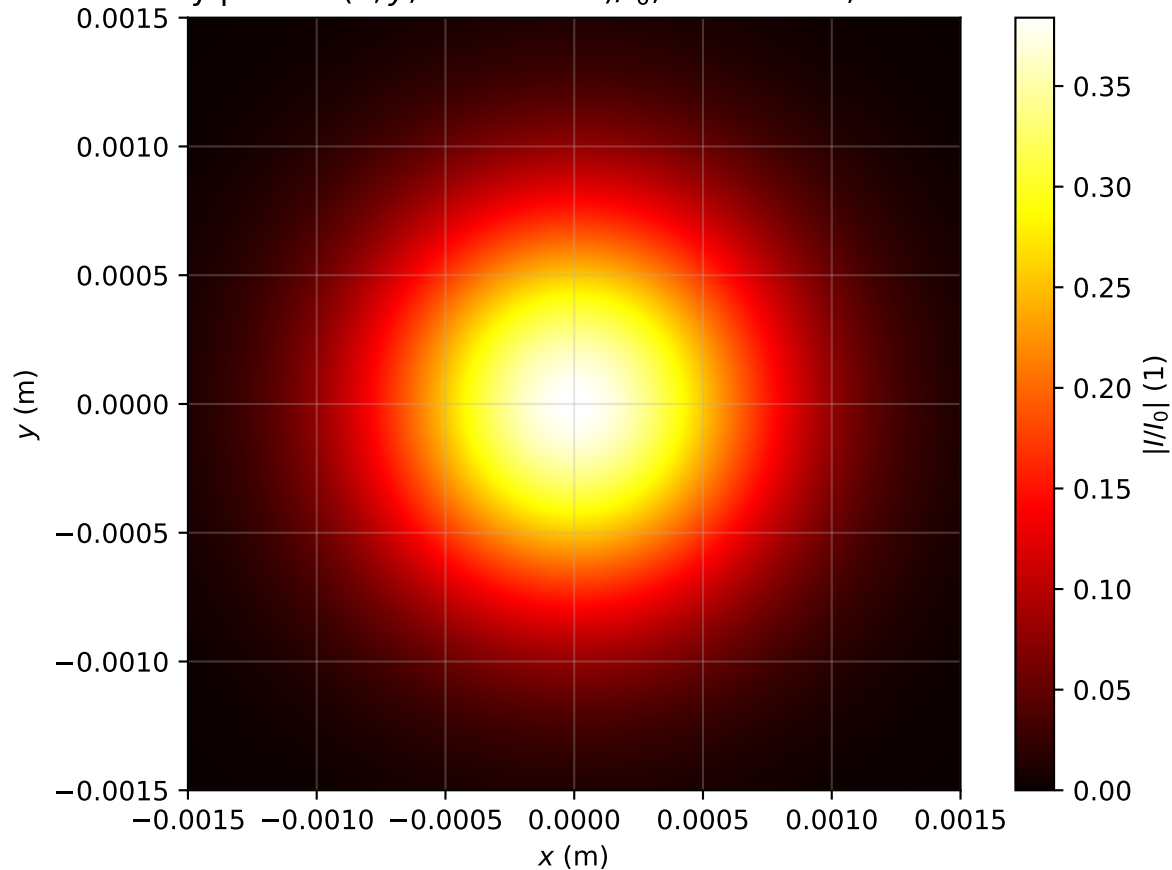
Intensity profile I(x, y, z = 2.946m)/I_0 , P_{in}=0.2P_{cr} , artificial time
